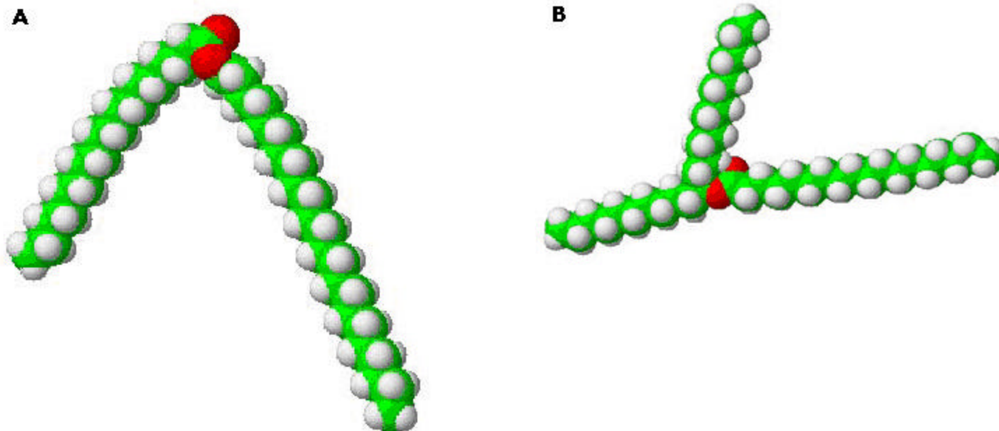
Figure 8. Space-filling models for (A) tricosanyl 1-stearate and (B) tricosanyl 11-stearate. The latter is the major wax ester species found on the cuticle of M. sanguinipes (Blomquist et al. , 1972). Green atoms are carbons, red atoms are oxygens, and gray atoms are hydrogens.
