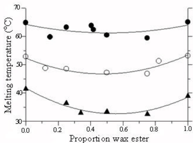
Figure 7. Melting temperatures of mixtures containing a wax ester and an n -alkane. Filled circles: stearyl arachidate (C18:0-20:0) and triacontane (C30); open circles: tetradecyl stearate (C14:0-18:0) and pentacosane (C25); filled triangles: dodecyl myristate (C12:0-14:0) and heneicosane (C21).
