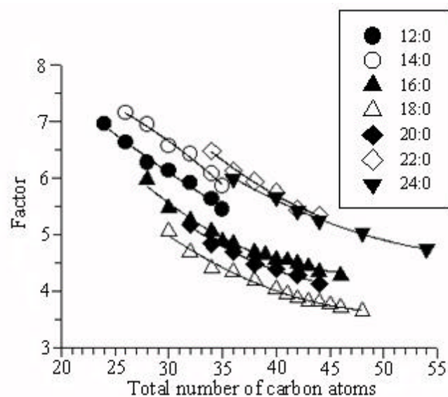
Figure 1. The effects of wax ester chain length and size of the acid and alcohol moieties on the factor needed to convert SIM values for the protonated acid fragment to TIC values for the wax ester.
