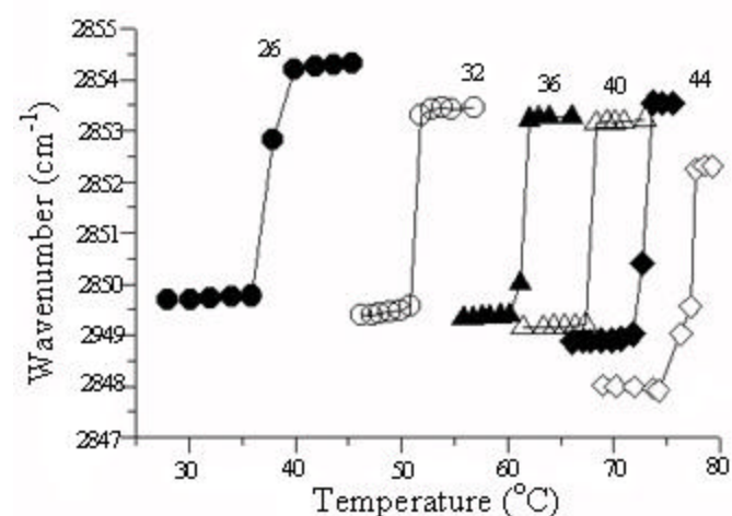
Figure 2. Melting curves for saturated wax esters. At the T_m , the symmetric stretching frequency of -CH 2 - groups of acid chains increases from ~2850 cm -1 to ~2854 cm -1 . Numbers indicate the total number of carbon atoms in each molecule. Except for the shortest wax (C12:0-14:0), each compound had an equal number of carbons in the alcohol and fatty acid moieties.
